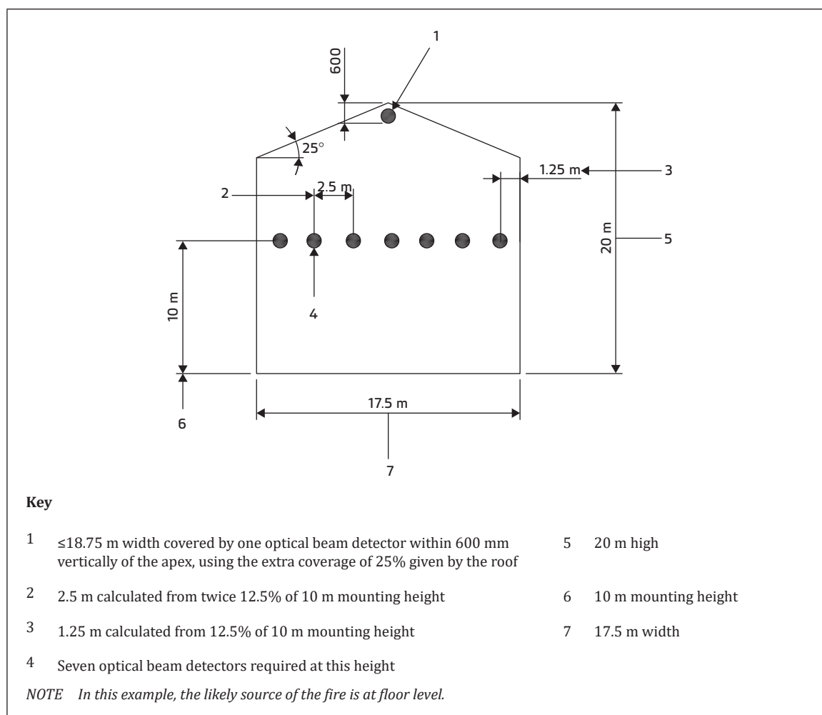
Figure 16 — Siting optical beam detectors
