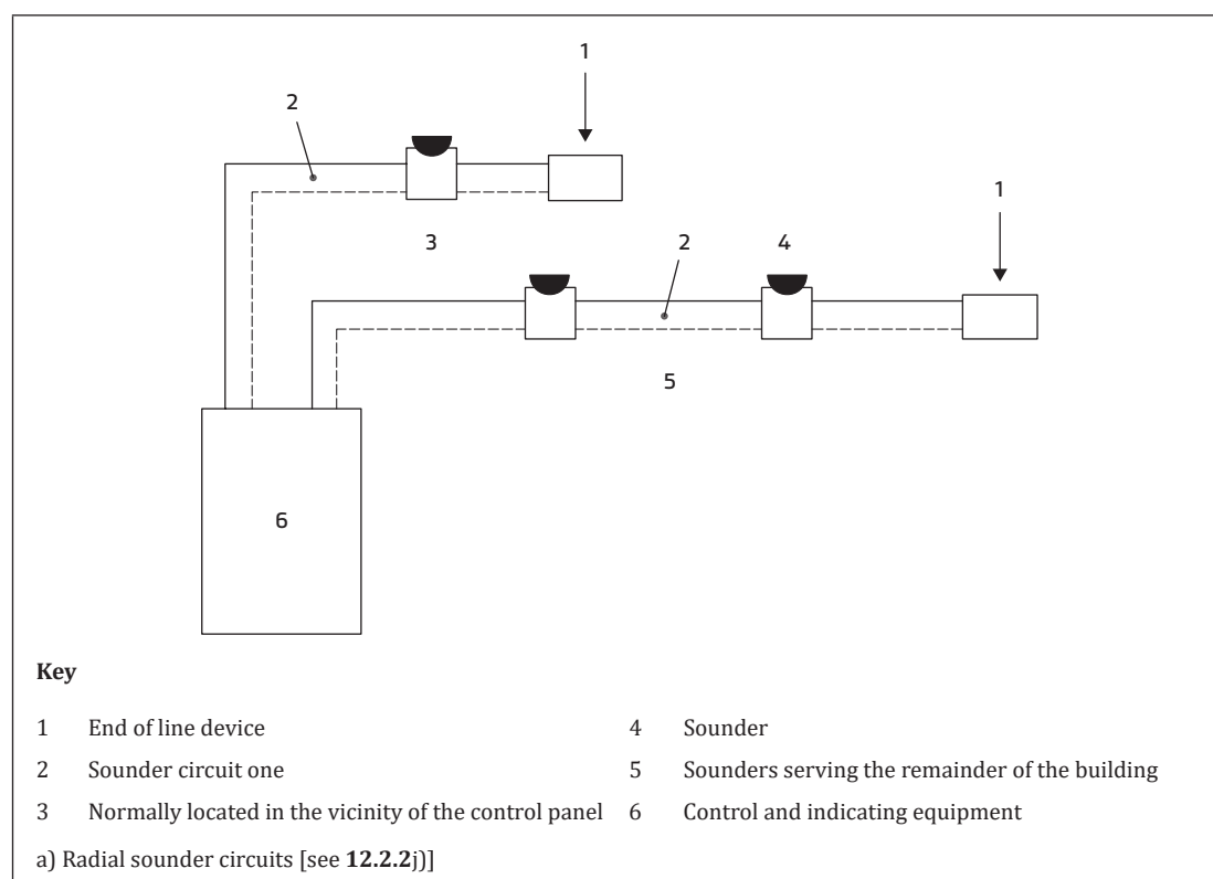
Figure 1 — Sounder circuits
