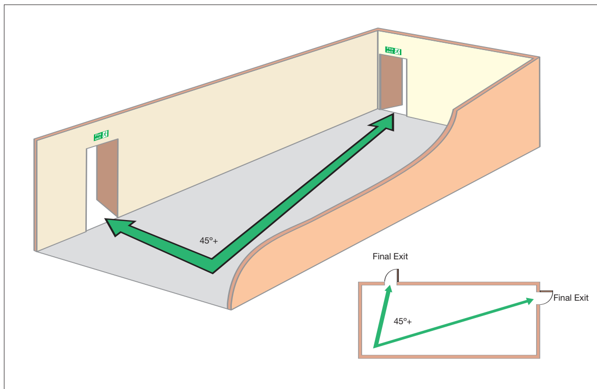
Figure 23: Alternative exits
