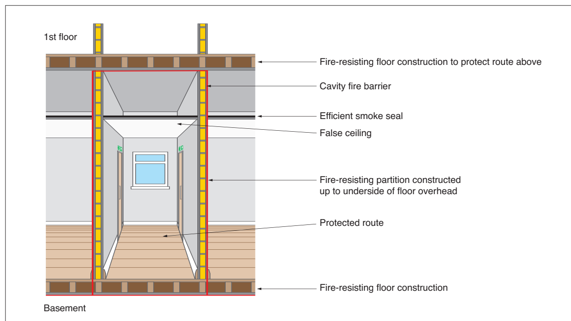
Figure 60: Fire-resisting construction
