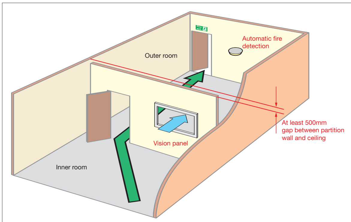
Figure 22: Inner rooms
