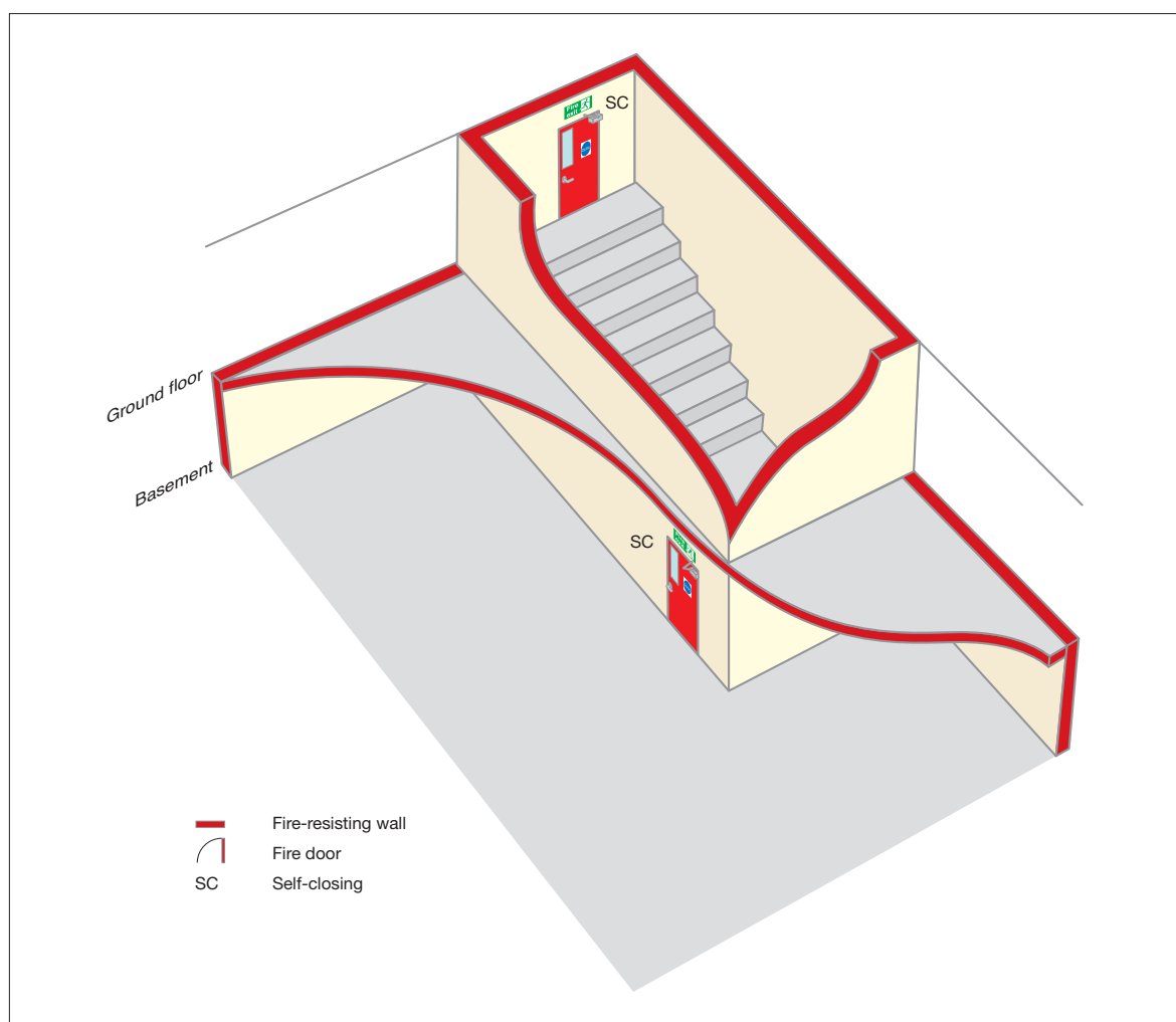
Figure 30: Basement protection
