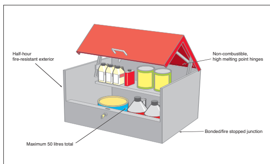
Figure 15: A 50-litre flammable storage bin
