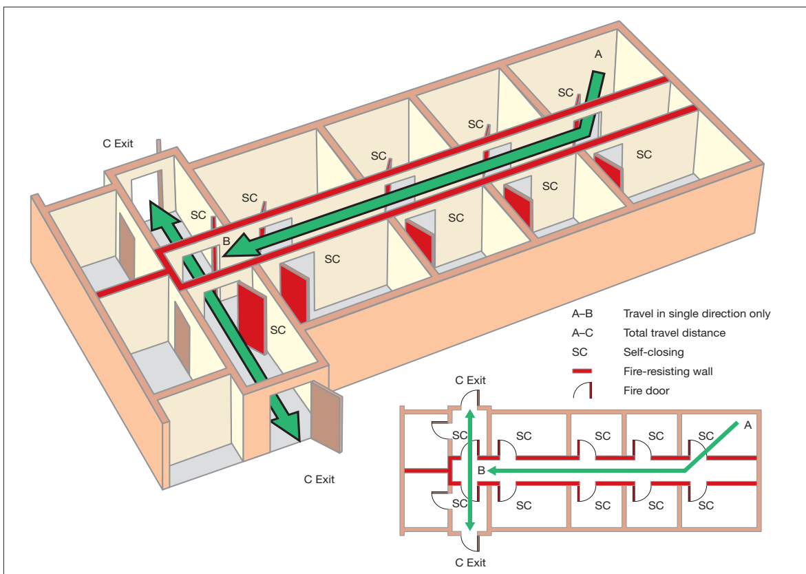
Figure 30: Dead-end condition with fire-resisting construction
